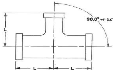
Shouldered unequal Tee
