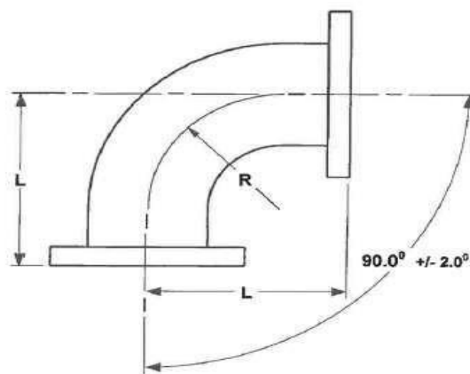
Flanged 90° Bend (SANS 1123 Table 1600/3)
