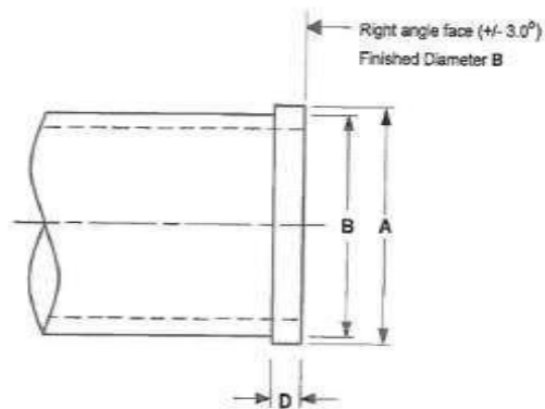
Shouldered end
