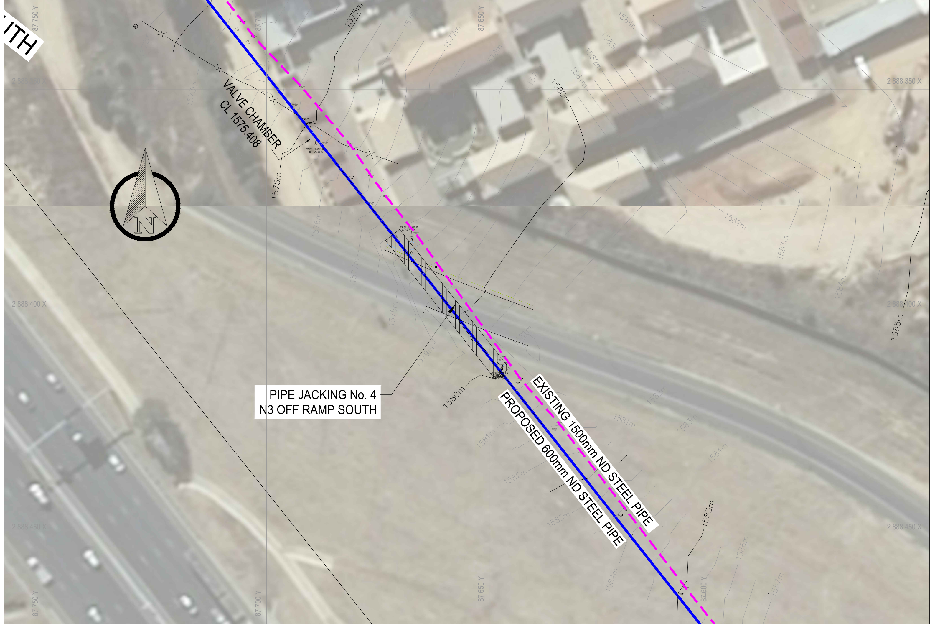
PLAN OF PIPE JACKING No. 4 UNDER N3 OFF RAMP SOUTH SCALE 1:500
