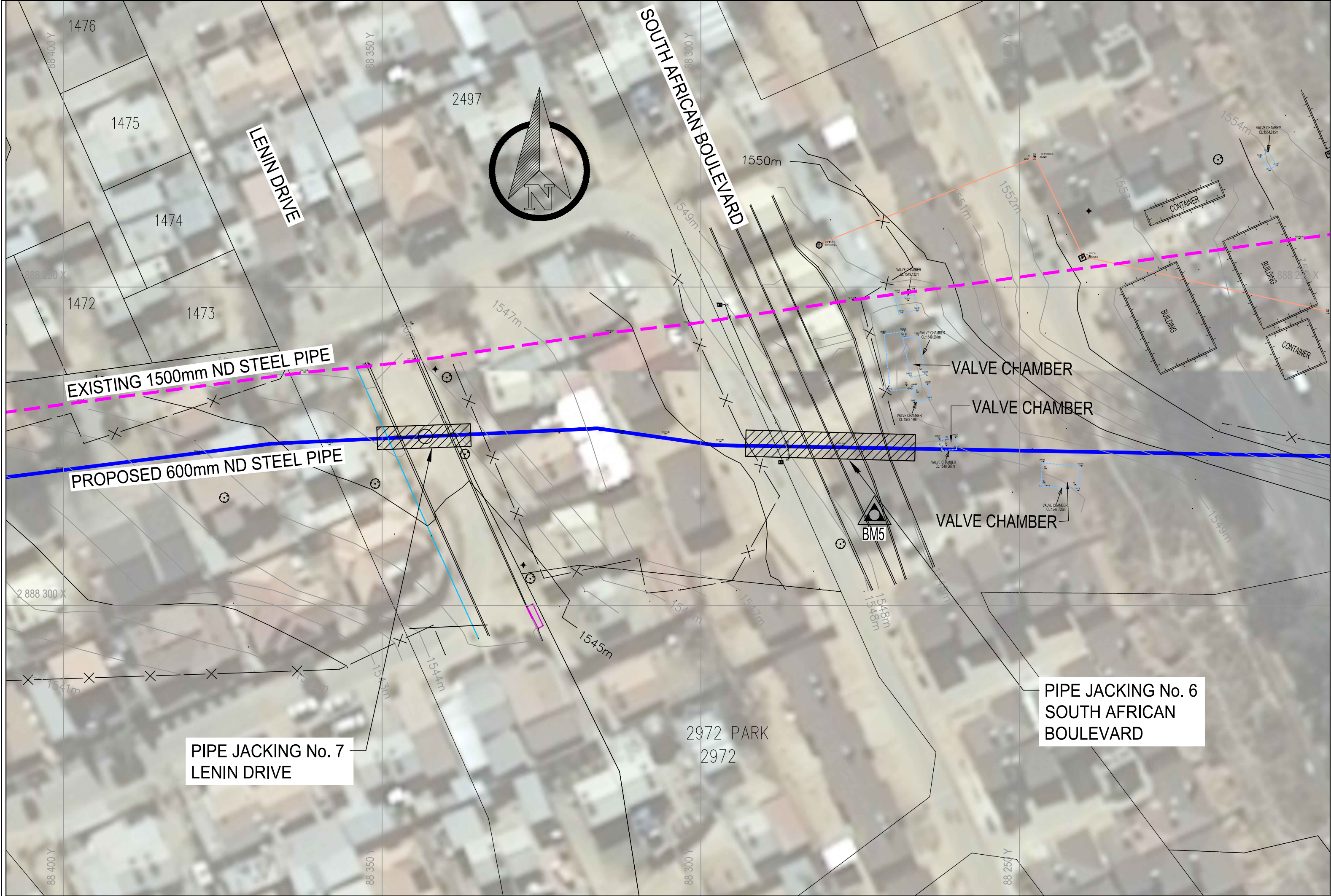
PLAN OF PIPE JACKING No. 6 & 7 UNDER SOUTH AFRICAN BOULEVARD & LENIN DRIVE SCALE 1:500
